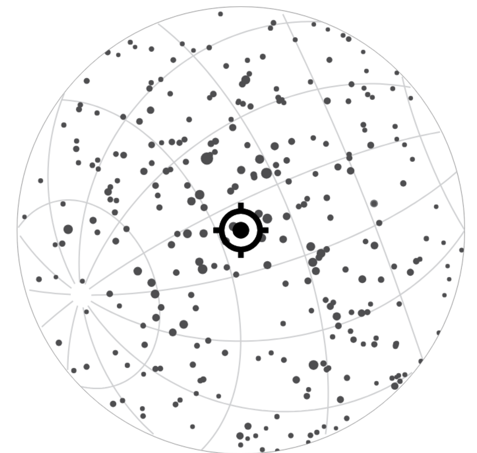
Polar Projection
