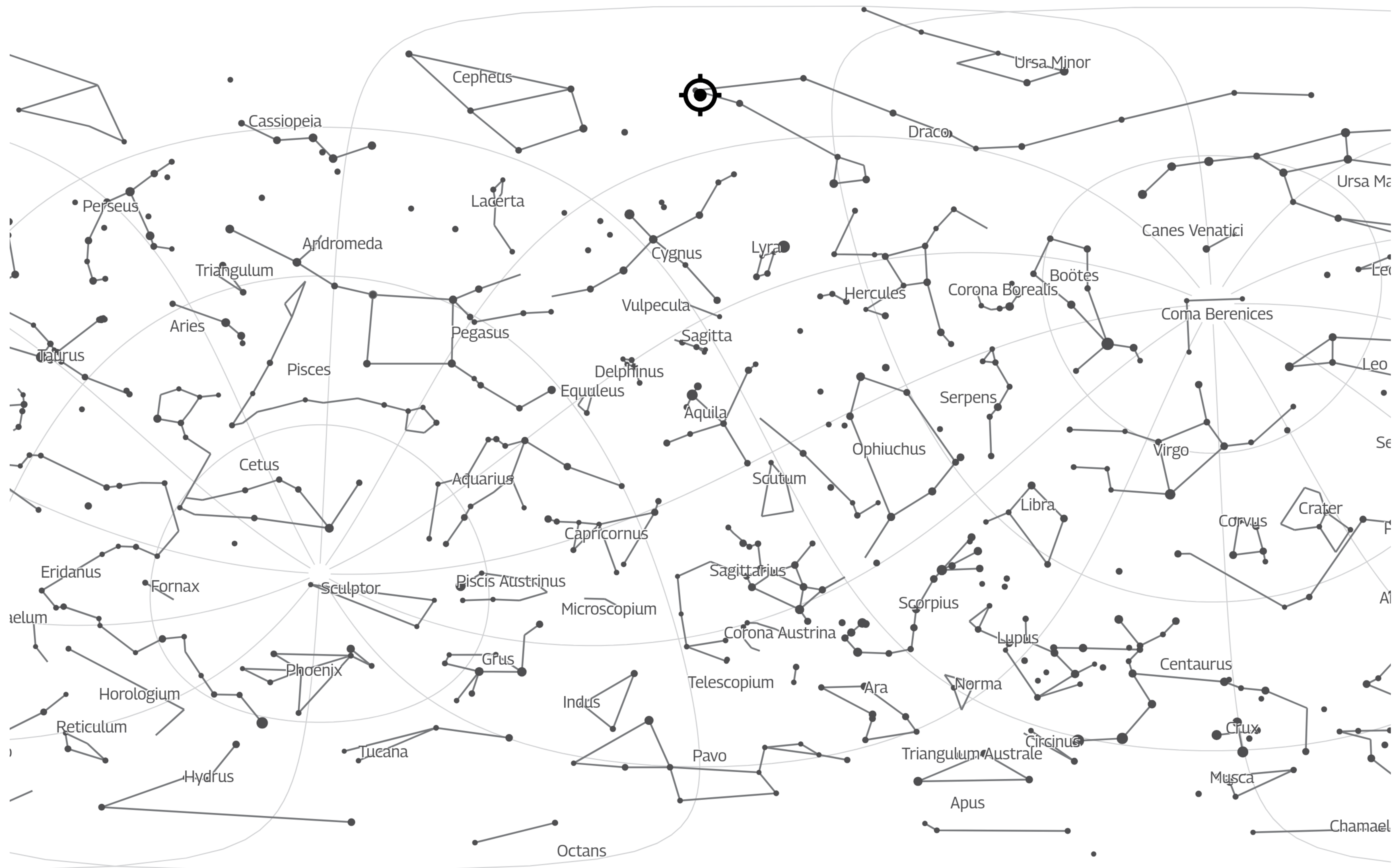
Equirectangular Projection
